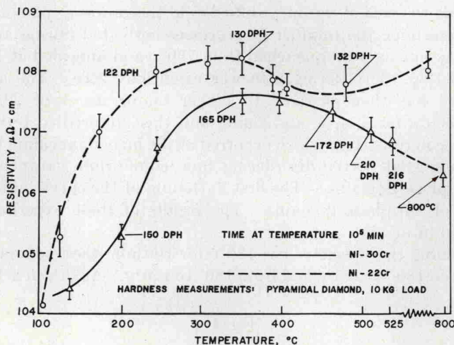
Effect of long time anneals on the final resistivity and hardness of Ni-22 Cr and Ni-30 Cr.
